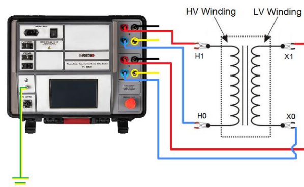
Connecting TRT400 to a single-phase transformer
