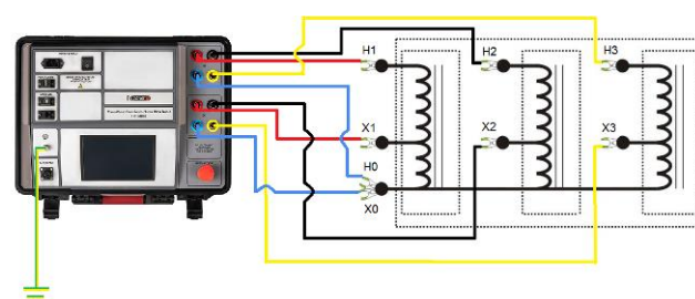
Connecting TRT400 to a three-phase autotransformer
