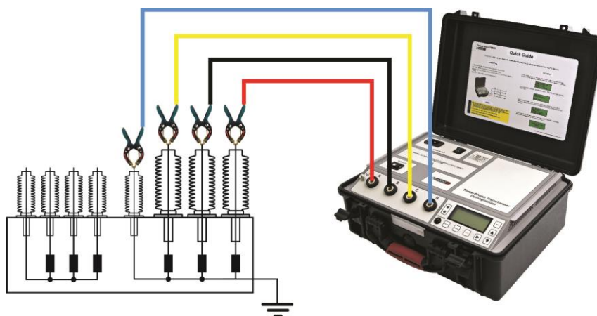
Connecting DEM60R to a three-phase transformer
